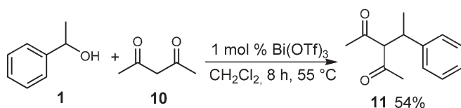
Scheme 4. Bi(OTf) 3 -catalyzed alkylation of acetylacetone.
