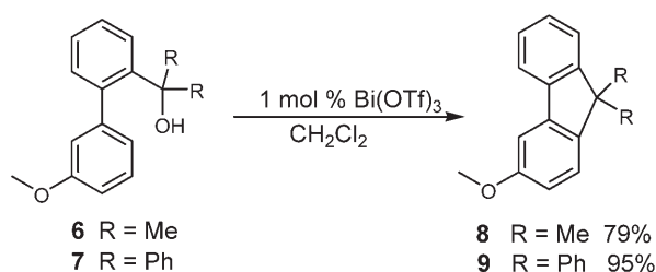
Scheme 3. Intramolecular Bi(OTf) 3 -catalyzed arylation.
