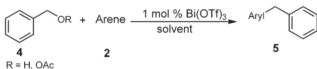
Scheme 2. Bi(OTf) 3 -catalyzed reaction of arenes with benzyl alcohol and benzyl acetate.
